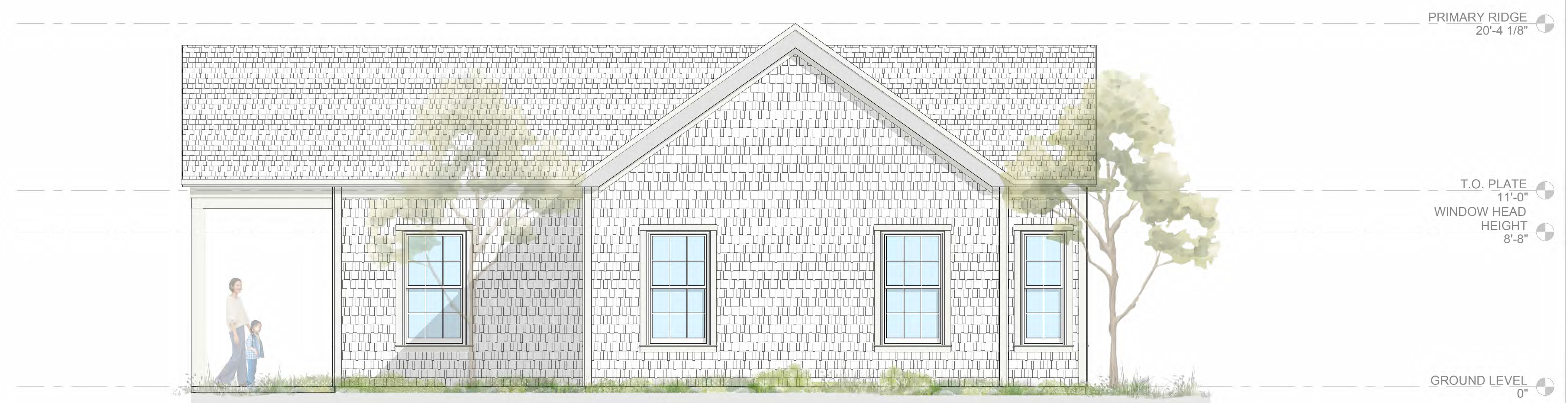
2 BUILDING ELEVATION - SOUTH 1/4" = 1'-0"
