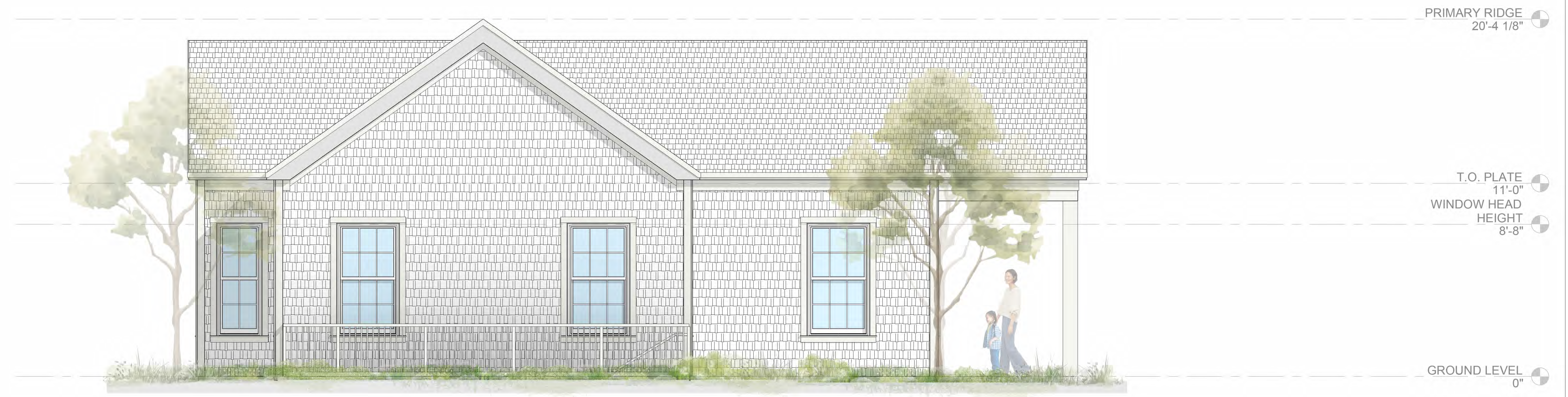
1 BUILDING ELEVATION - NORTH 1/4" = 1'-0"
