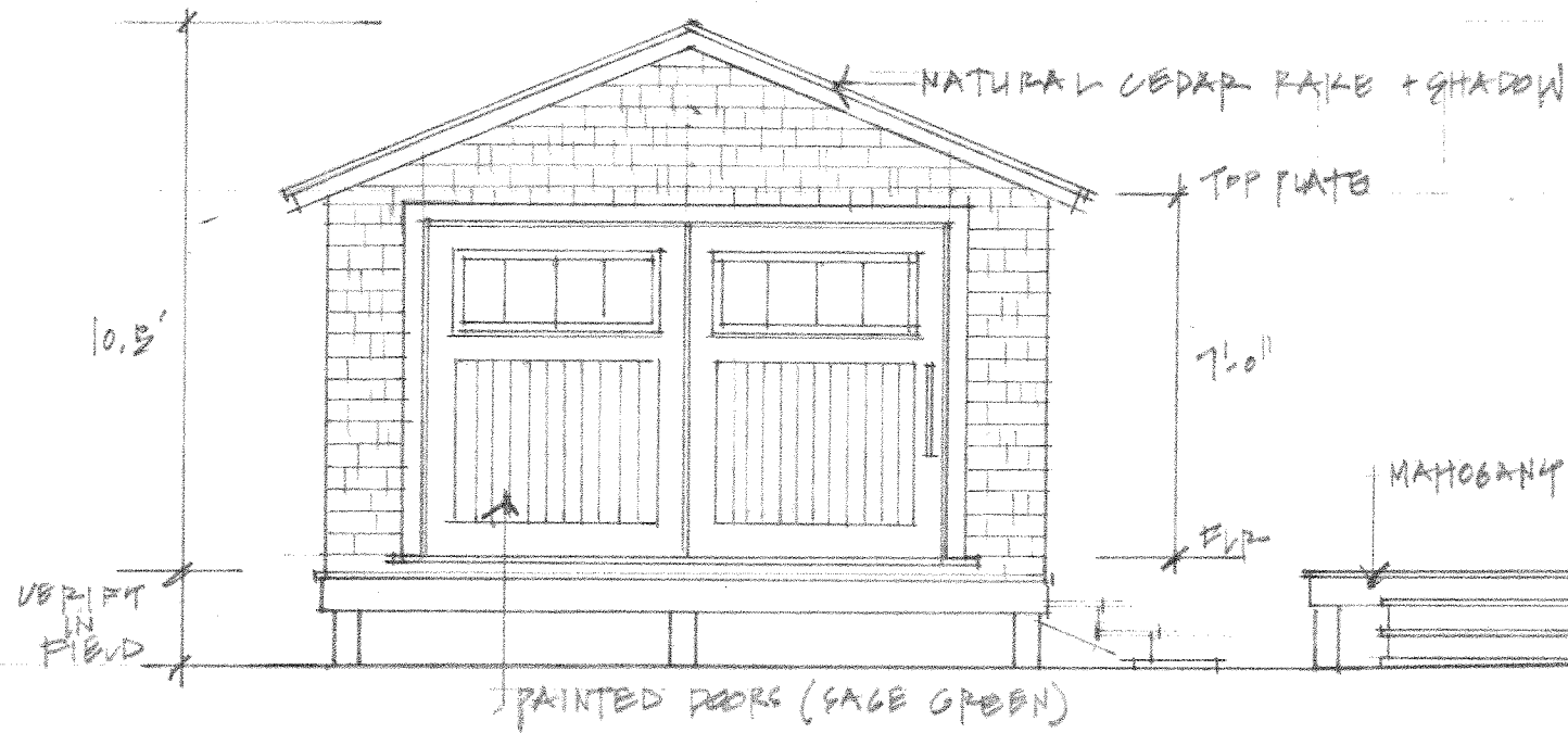
SOUTH ELEVATION (POND)
