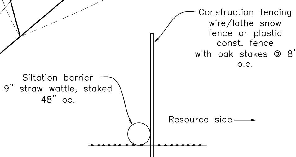
Silt/Const. Barrier Detail no scale
