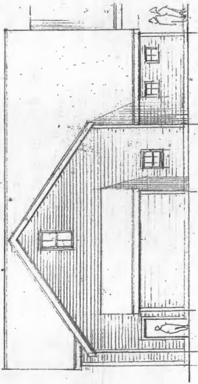
SOUTH ELEVATION
