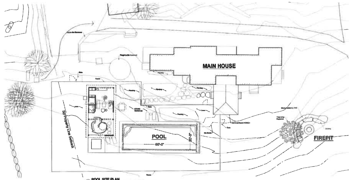
1 POOL SITE PLAN Scale 1/16" = 1'-0"
