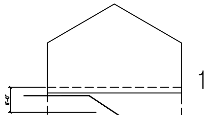
GRADE PLANE EXAMPLES. RE: STORY ABOVE GRADE PLANE, ALTERNATE 1
