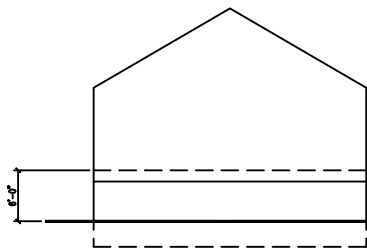
GRADE PLANE EXAMPLES. RE: STORY ABOVE GRADE PLANE, ALTERNATE 1
