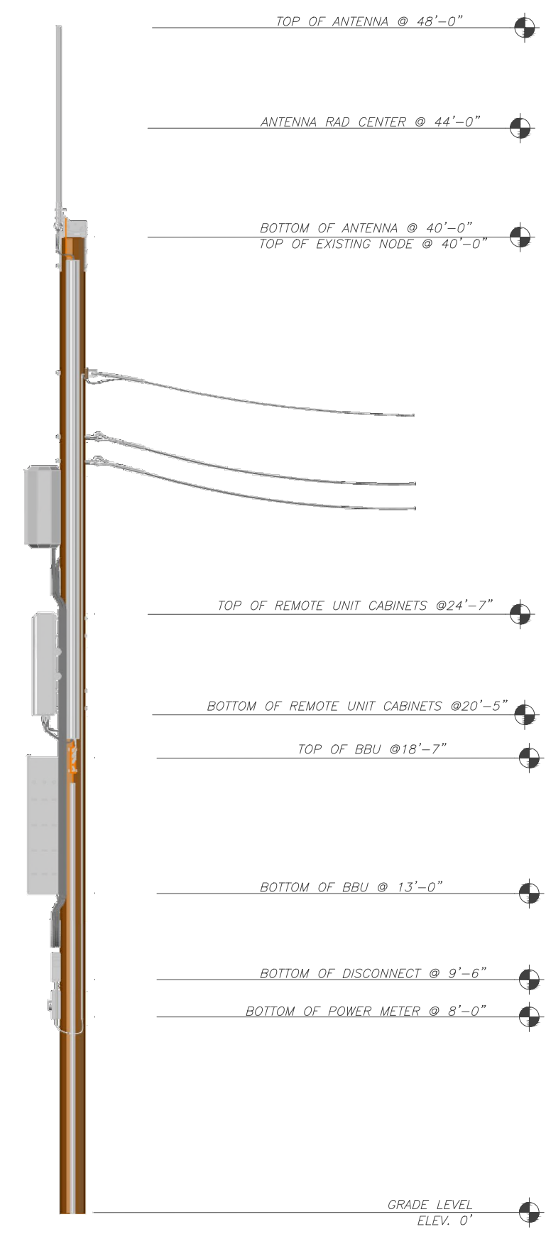
2 TYPICAL NODE ELEVATION (SIDE) SCALE: NOT TO SCALE
