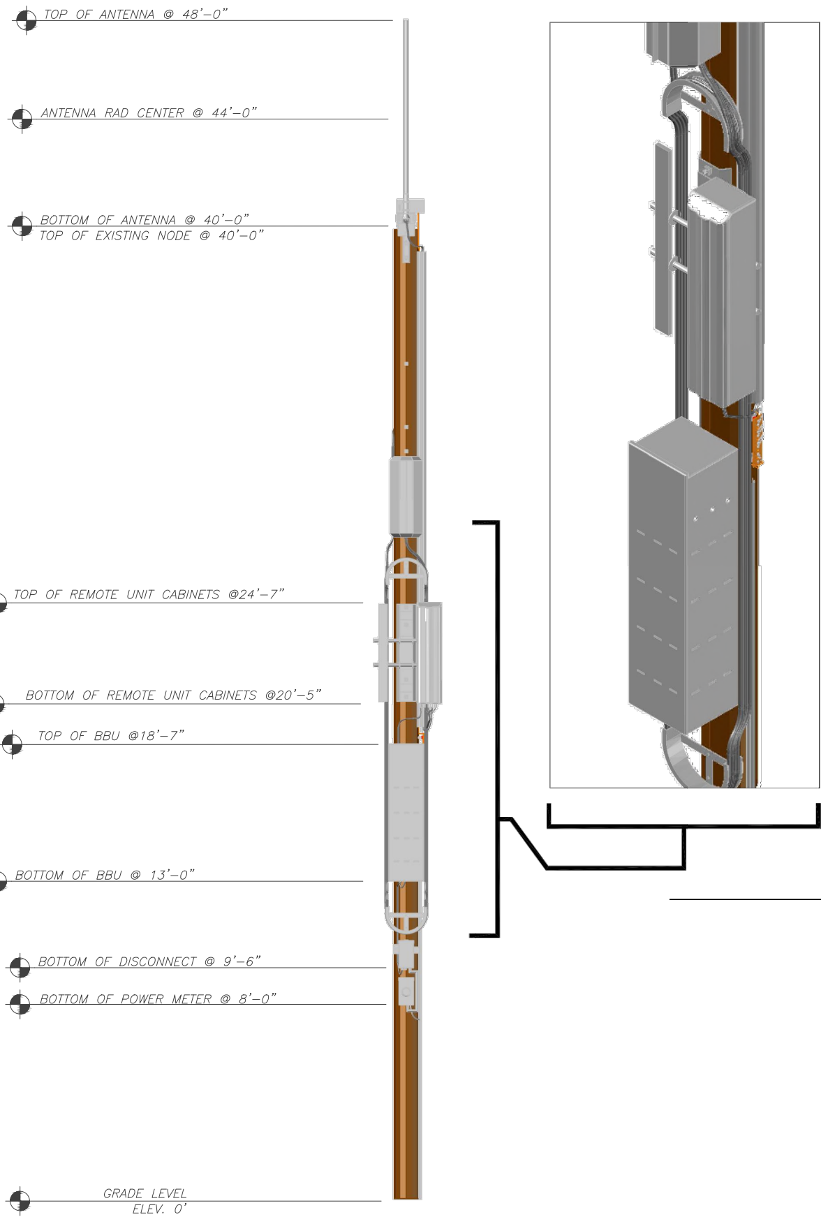
1 TYPICAL NODE ELEVATION (FRONT) SCALE: NOT TO SCALE
