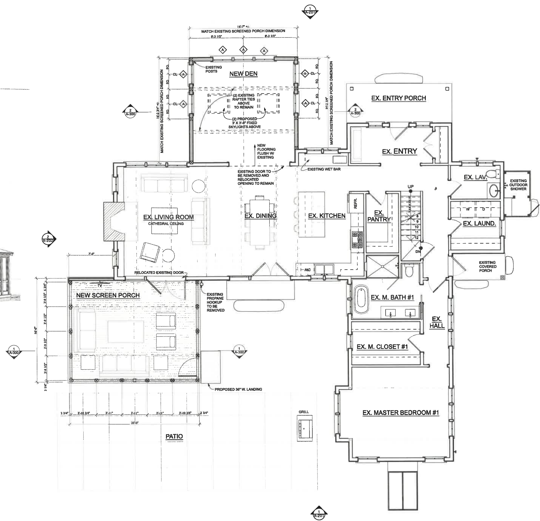
FIRST FLOOR PLAN - PROPOSED SCALE 1/4" = 1'-0"
