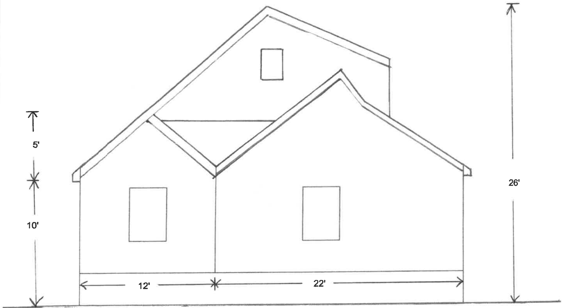
Proposed Elevation
